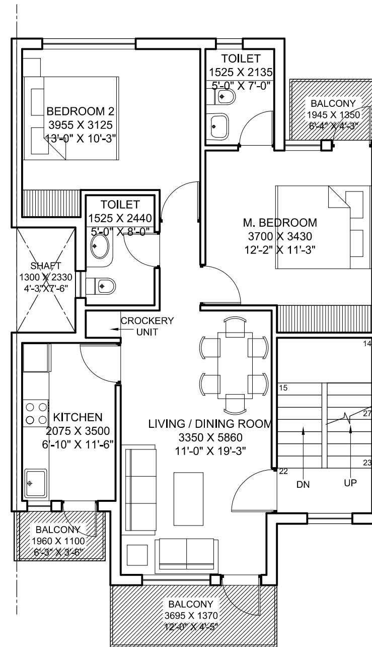
FIRST FLOOR PLAN REVISED OPTION
