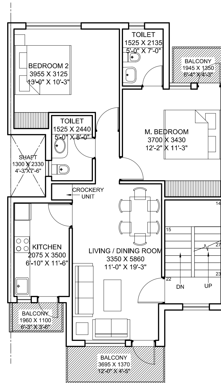
SECOND FLOOR PLAN REVISED OPTION
