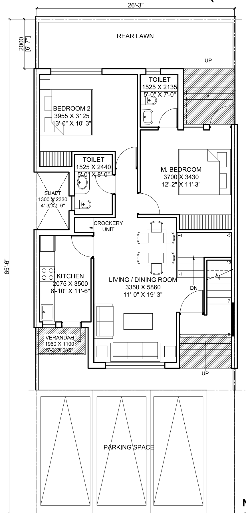
GROUND FLOOR PLAN REVISED OPTION
