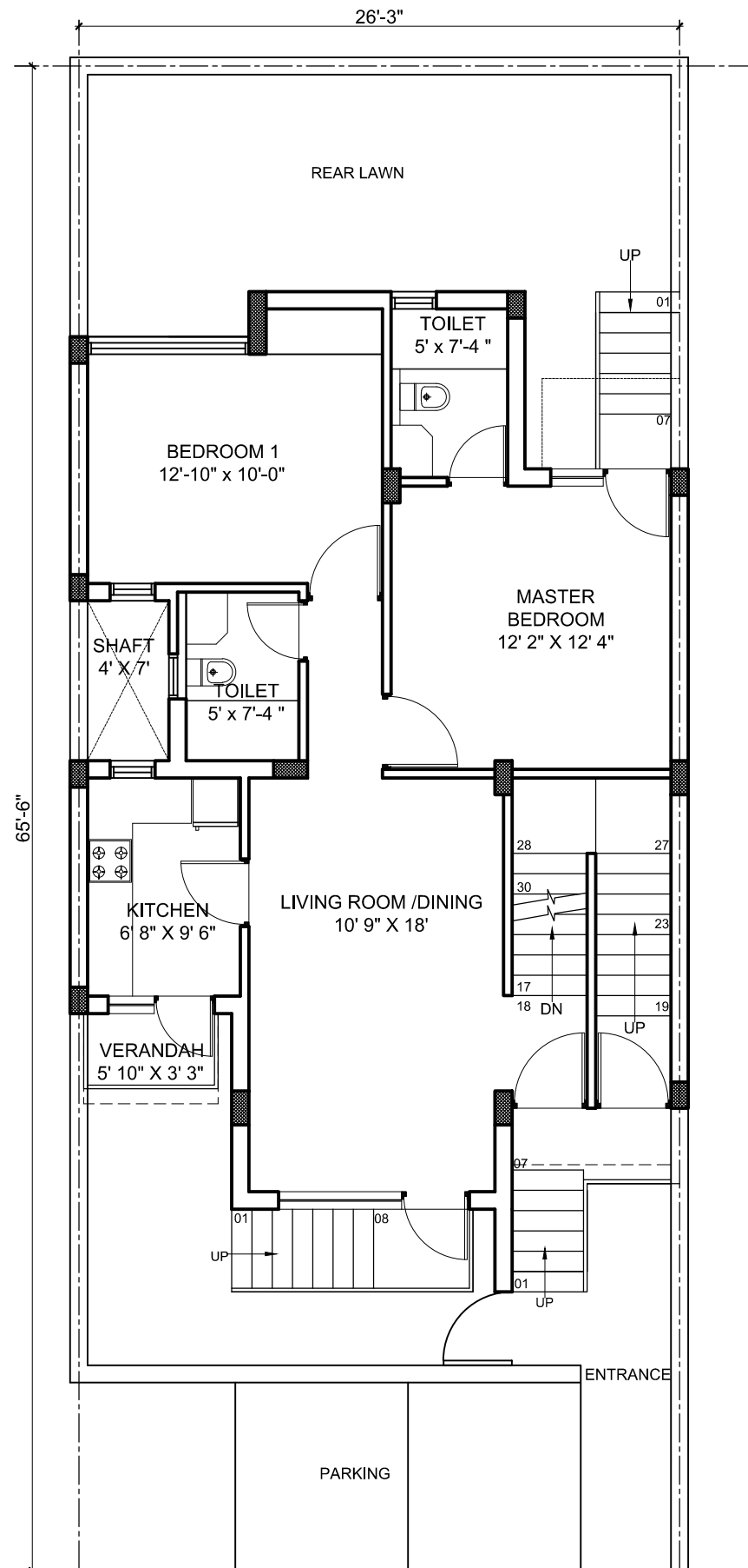
GROUND FLOOR PLAN ORIGINAL OPTION
