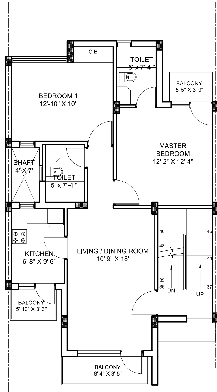
FIRST FLOOR PLAN ORIGINAL OPTION
