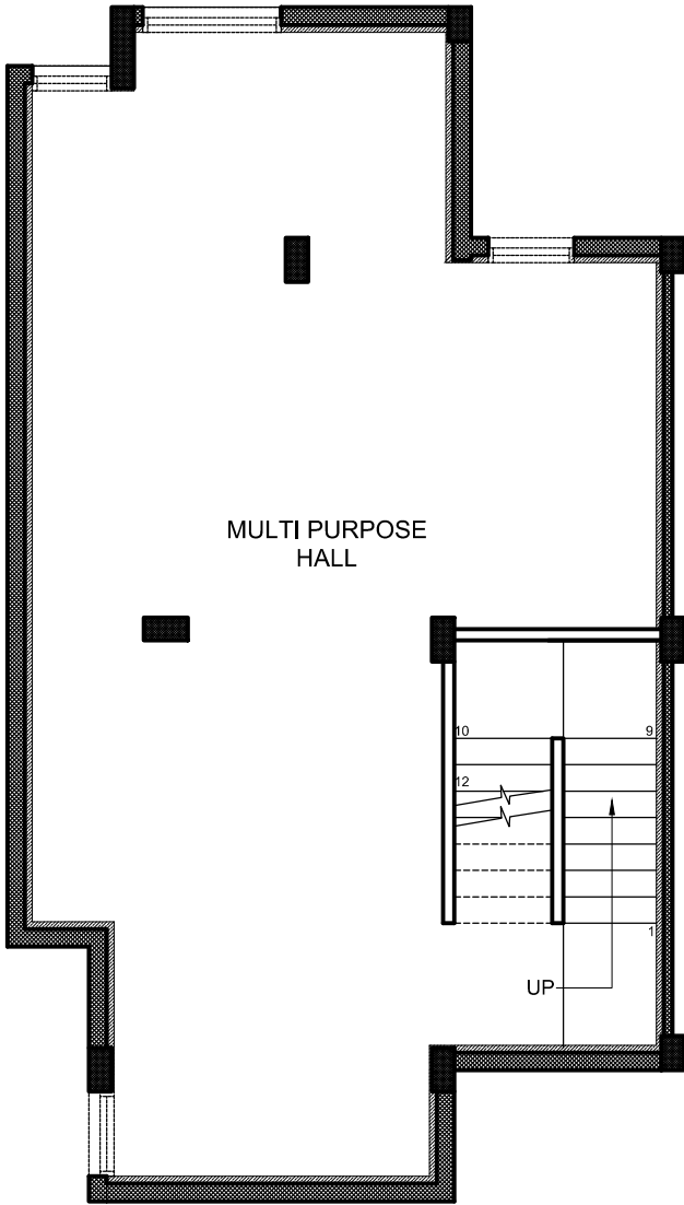
BASEMENT FLOOR PLAN ORIGINAL OPTION
