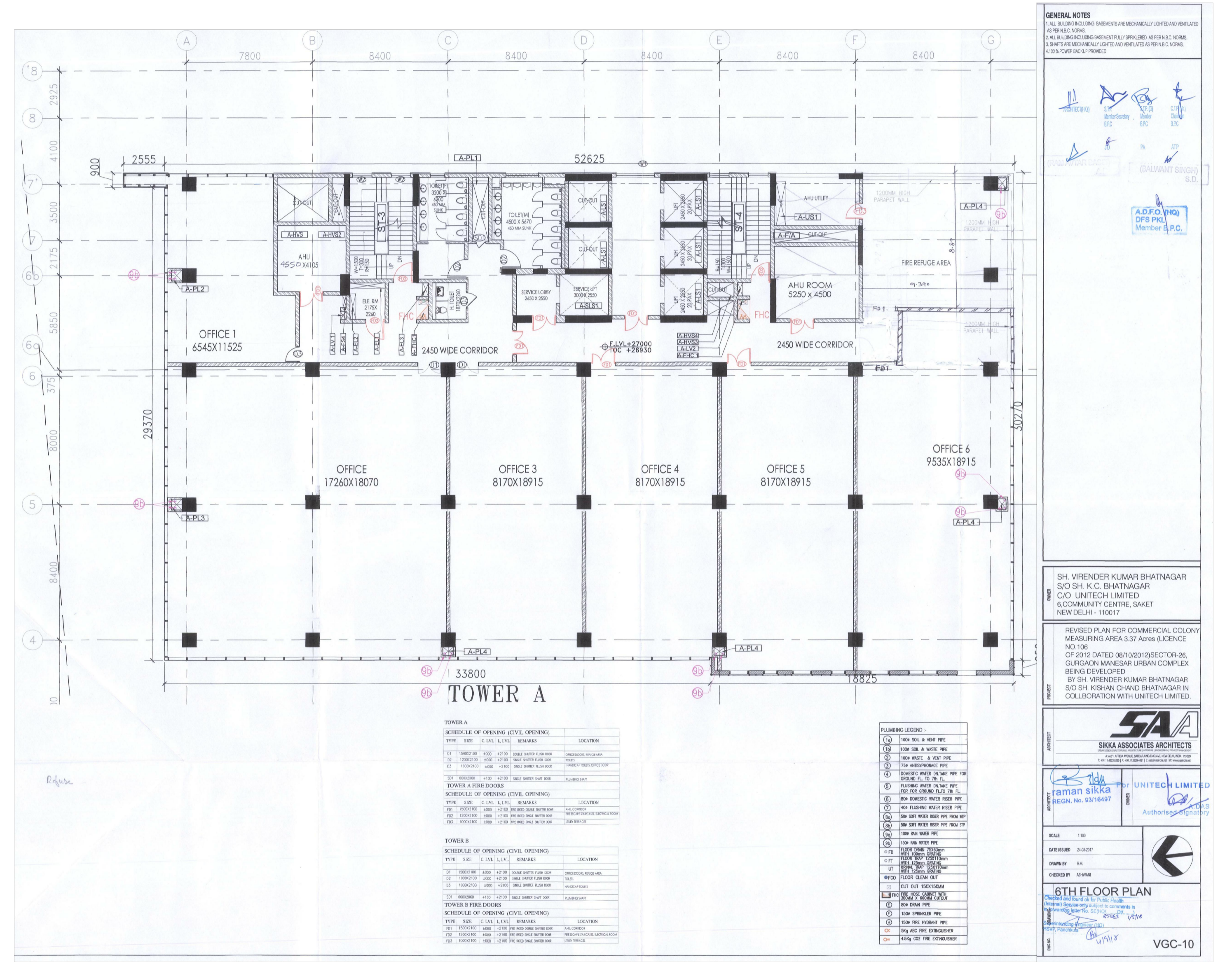
BLOCK - A , 6TH FLOOR PLAN
