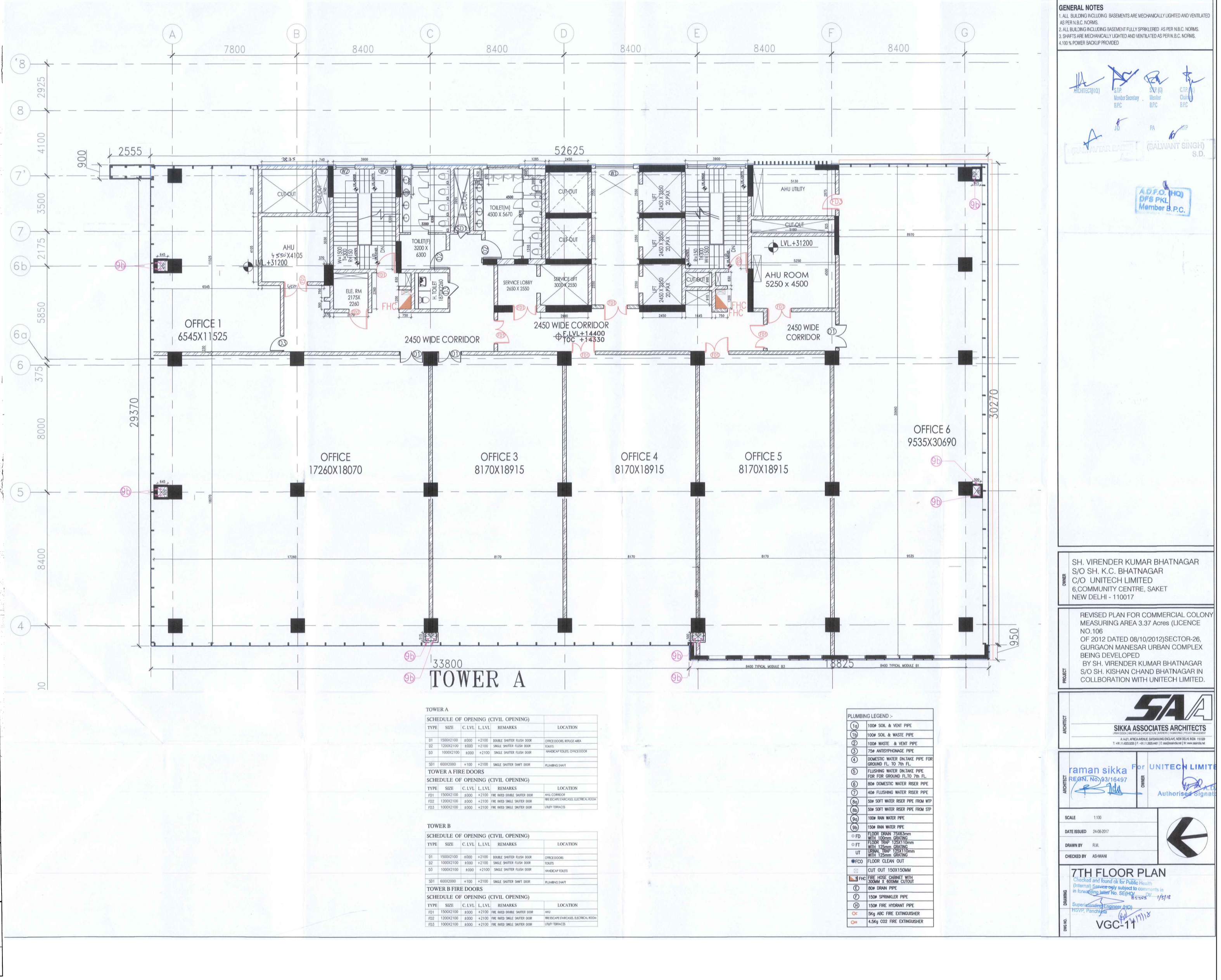
BLOCK - A , 7TH FLOOR PLAN
