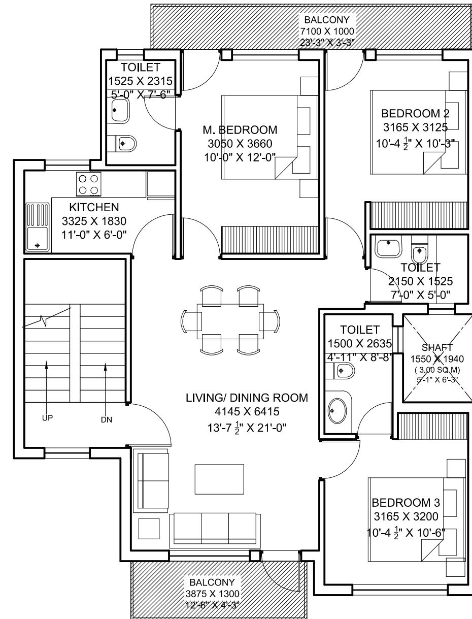
FIRST FLOOR PLAN REVISED OPTION
