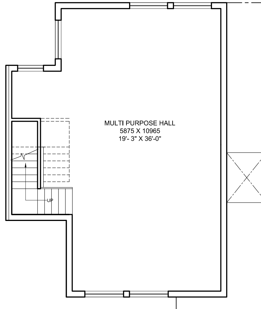
BASEMENT FLOOR PLAN REVISED OPTION
