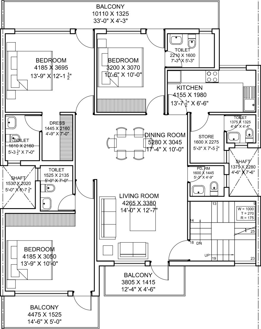
SECOND FLOOR PLAN REVISED OPTION 1
